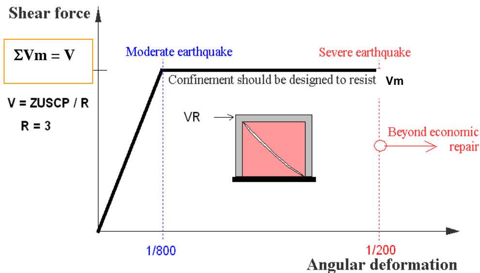
Figure 2. Objectives of the design procedure; V : Seismic design base shear; Z : Ground acceleration according to the zone; U : Building use factor; S : Soil factor; C : Building response coefficient; P : Building weight; R : Reduction factor = 3 for masonry (SENCICO 2003).
