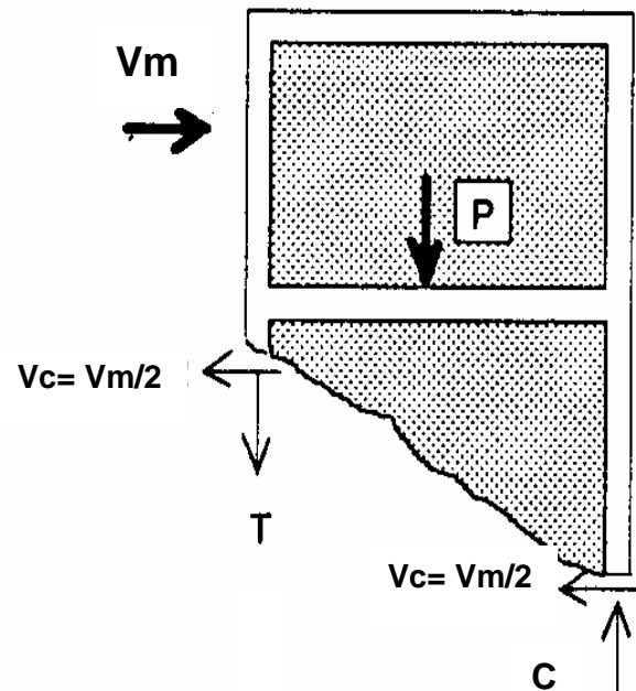
Figure 11. Vertical confinement internal forces of a one-bay wall
