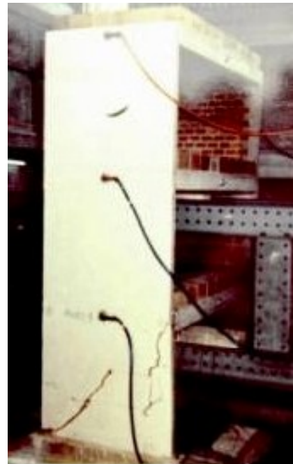
Figure 10. 3-story specimen tested on a shaking table.
